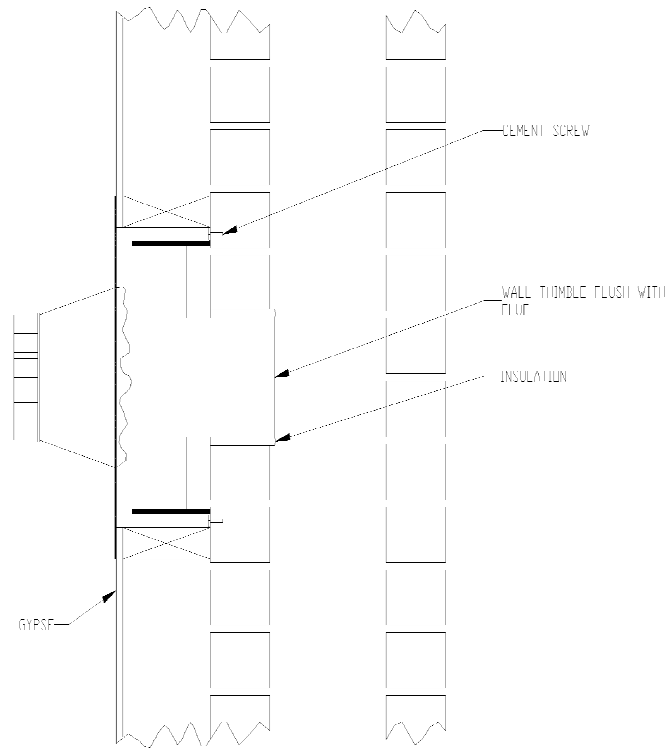
FIGURE 2.2.2 (B) Factory Built Thimble
