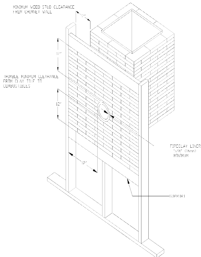
FIGURE 2.2.2 (C) Brick Thimble
