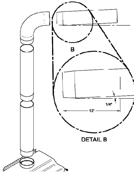
FIGURE 2.3 (B) Minimum Slope
